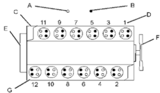
Illustration 1 (A) Inlet valves (B) Exhaust valves (C) Left side of the engine (D) Cylinder number (E) Front end of the engine (F) Front of the engine (G) Right side of the engine
