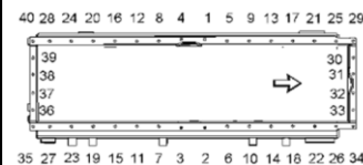
Illustration 4 Tightening Sequence The directional arrow is towards the front housing of the engine.
