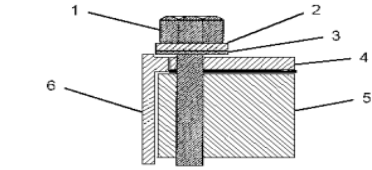
Illustration 1 Liner Projection Components (1) Bolt (2) Washer (3) Washer (4) Spacer plate (5) Block (6) Cylinder liner
